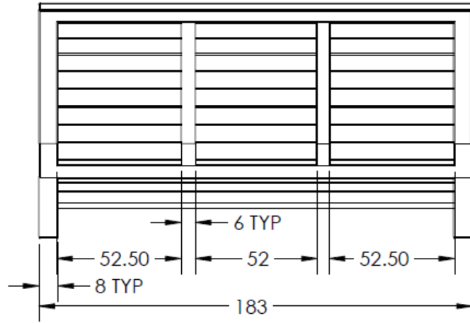
BACK VIEW SCALE 1:2
